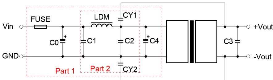
Figure 2. Circuit for EMC enhancement
