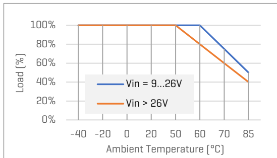
MU40G-24xx, and V_{OUT}=3.3V, 5V
