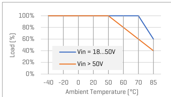
MU40G-48xx, and V_{OUT}=3.3V, 5V
