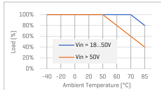
MU40G-48xx, and V_{OUT}=12 \dots 24V
